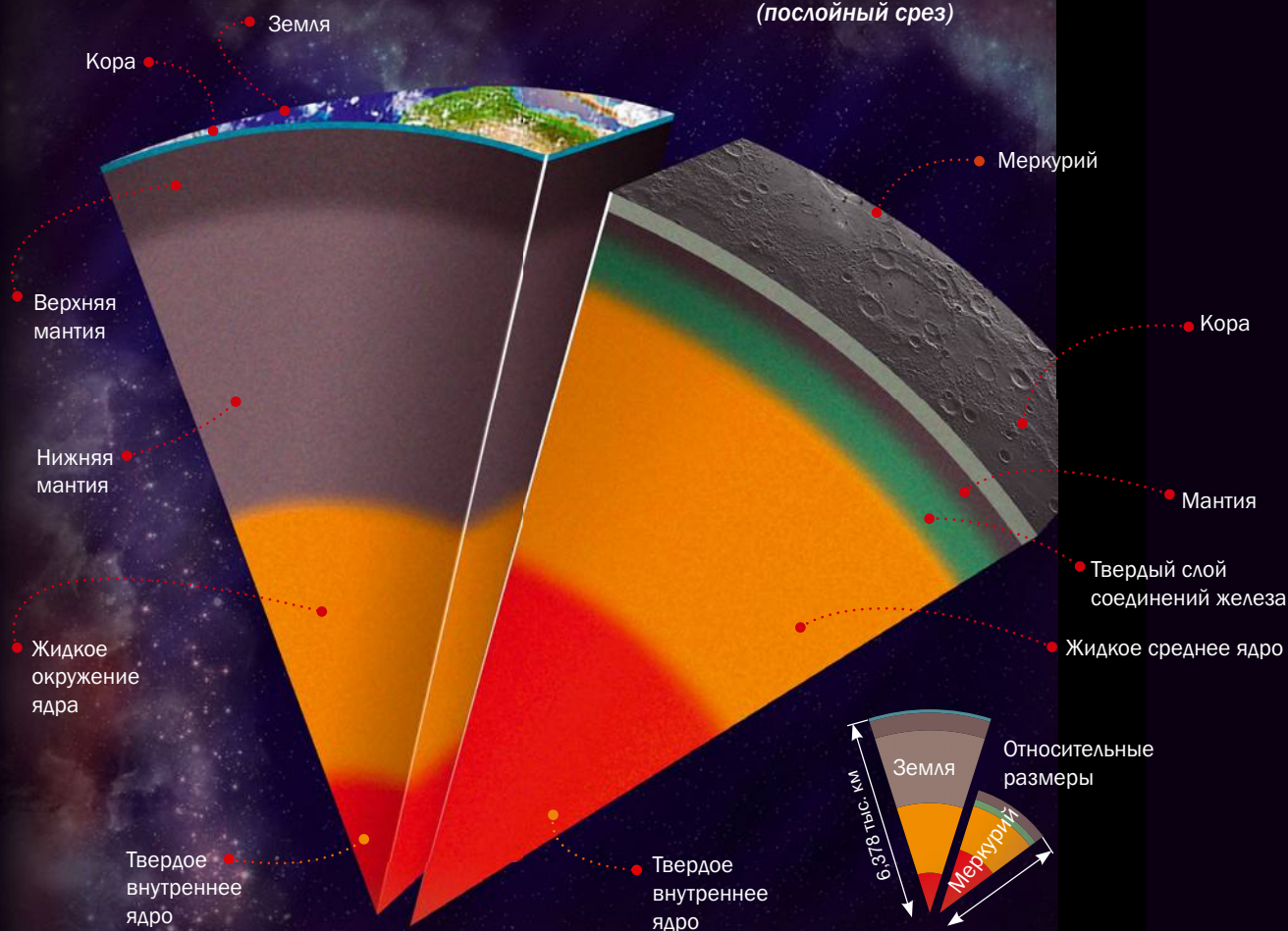
Mercury in comparison with Earth (cross-section)
